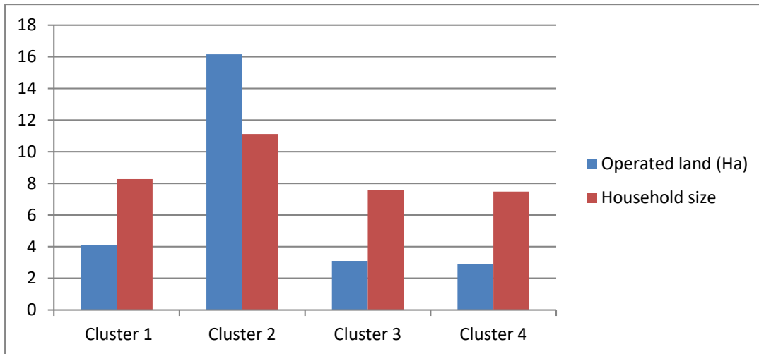
Figure 2: Land and family size across clusters.
