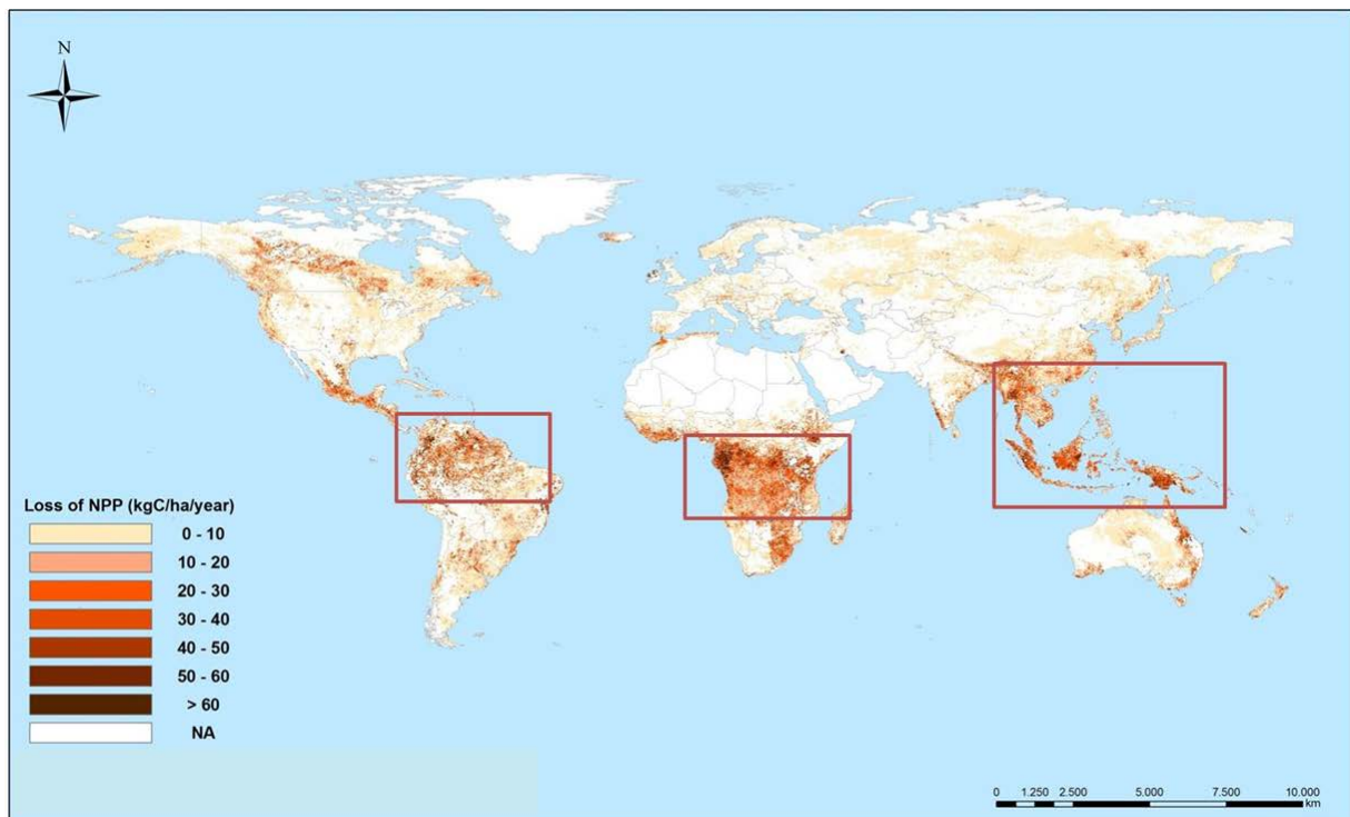
Figure 1. Loss of Net Primary Production between 1981-2003
