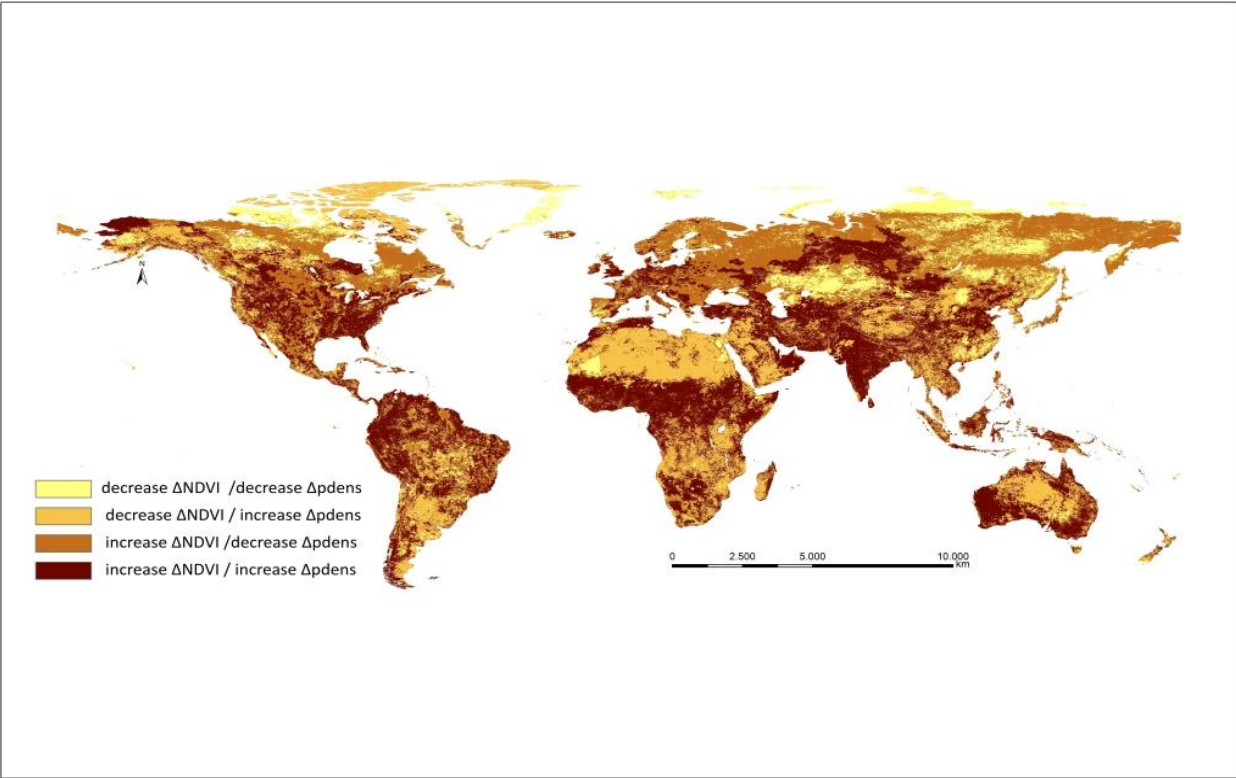
Figure 6. Relationship between NDVI and population density
