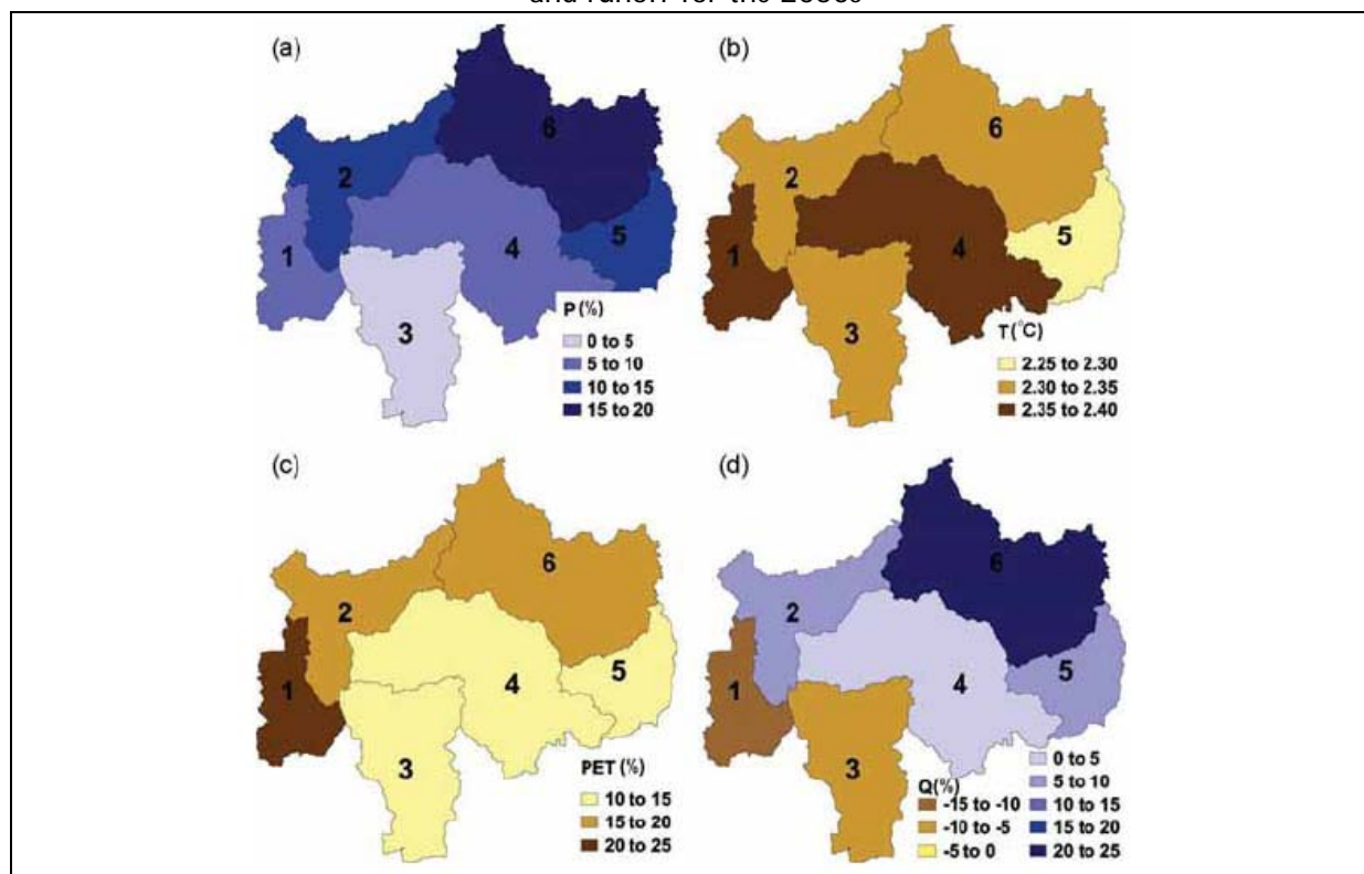
(a) Precipitation; (b) temperature, (3) potential evaporation; (d) runoff Source: Kim et al. 2008: 10
