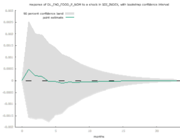
Figure A1: Different shocks on FAO food prices
